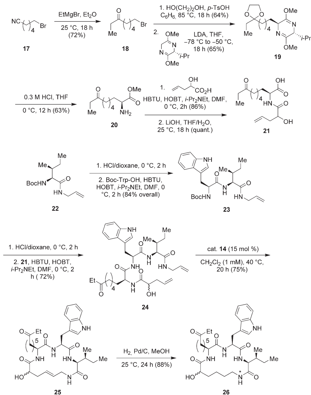
Scheme 4. Synthesis of apicidin analogues 25 and 26 .
