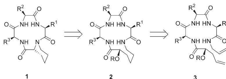
Scheme 1. Retrosynthesis of apicidin analogues.
