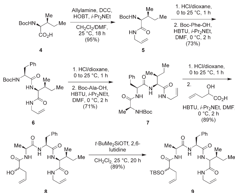
Scheme 2. Synthesis of peptide diene 9 . Boc = tert -butoxycarbonyl, DCC = N,N' -dicyclohexylcarbodiimide, HOBT = 1-hydroxybenzotriazole, HBTU = O -benzotriazol-1-yl- N,N,N',N' -tetramethyluronium hexafluorophosphate, Tf = trifluoromethanesulfonate.
