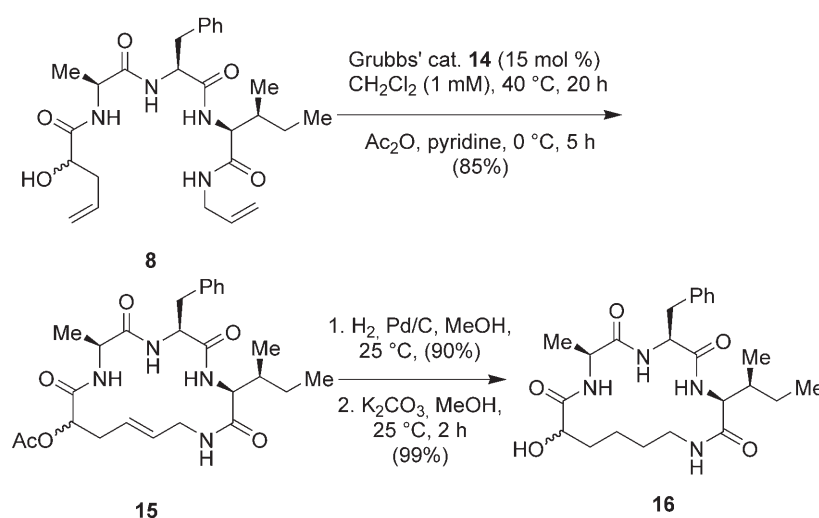
Scheme 3. Purification of macrocycle 16 via the acetate 15 .
